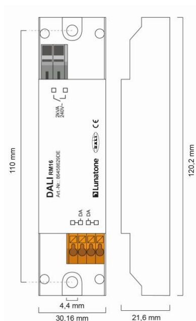
geometry RM16 DE
