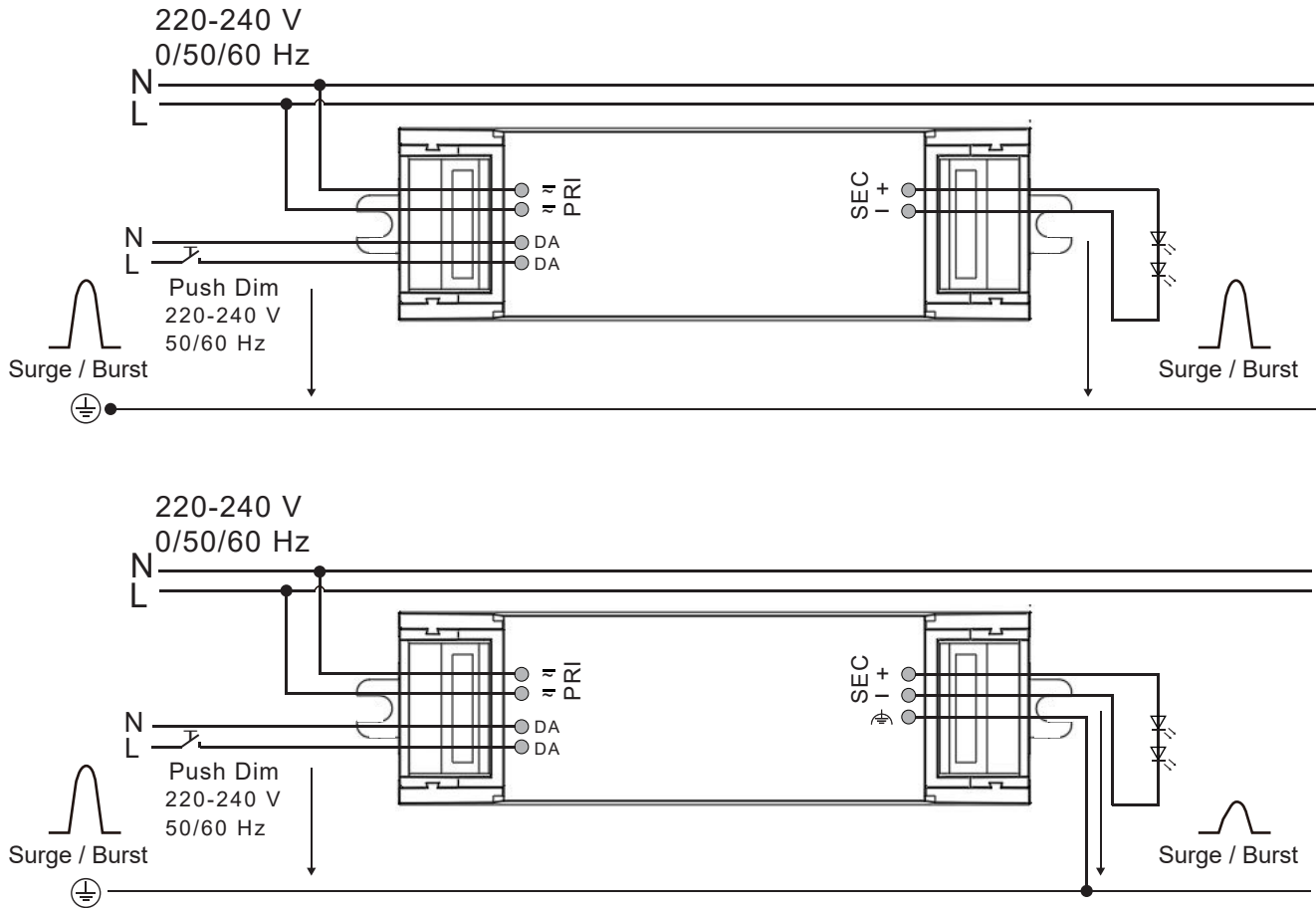
Figure: Voltage peaks for LED driver without earthing (Above) and with earthing (Below)
